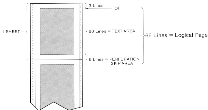
Figure 2-1 Text Area
