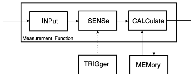
Figure 2-4 Expanded Measurement Function Model
