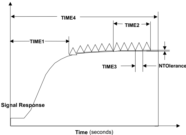
Figure 18.1 Stabilization Use
