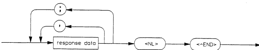
Figure 4-4. Simplified Response Message Syntax
