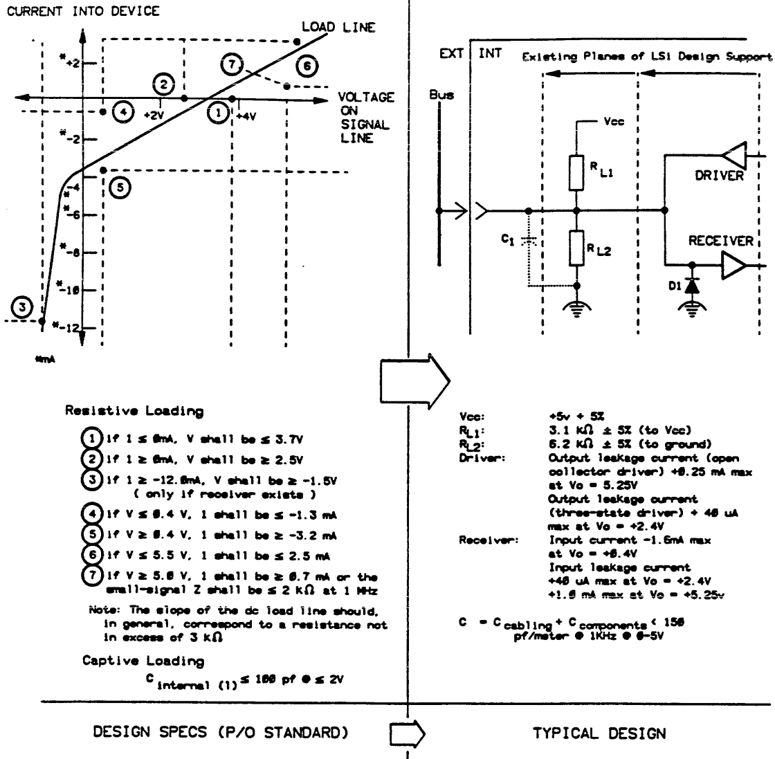
Figure 2.6 Converting Electrical Specifications to Actual Circuit
